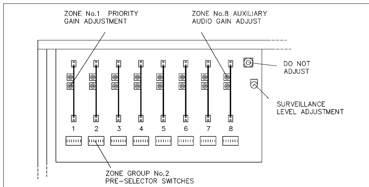
Fig. 7 Identification of output section components
