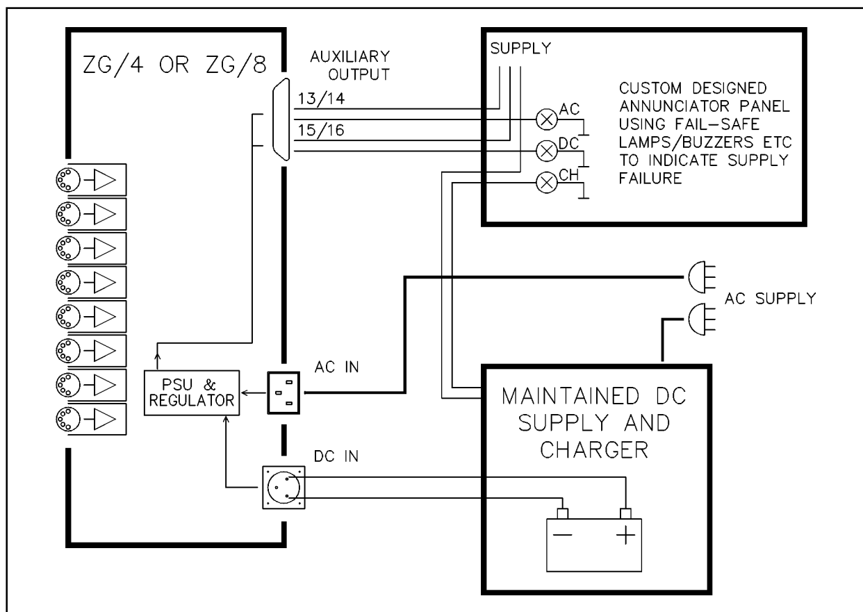
Fig. 10 AC & DC supply connections and monitoring
