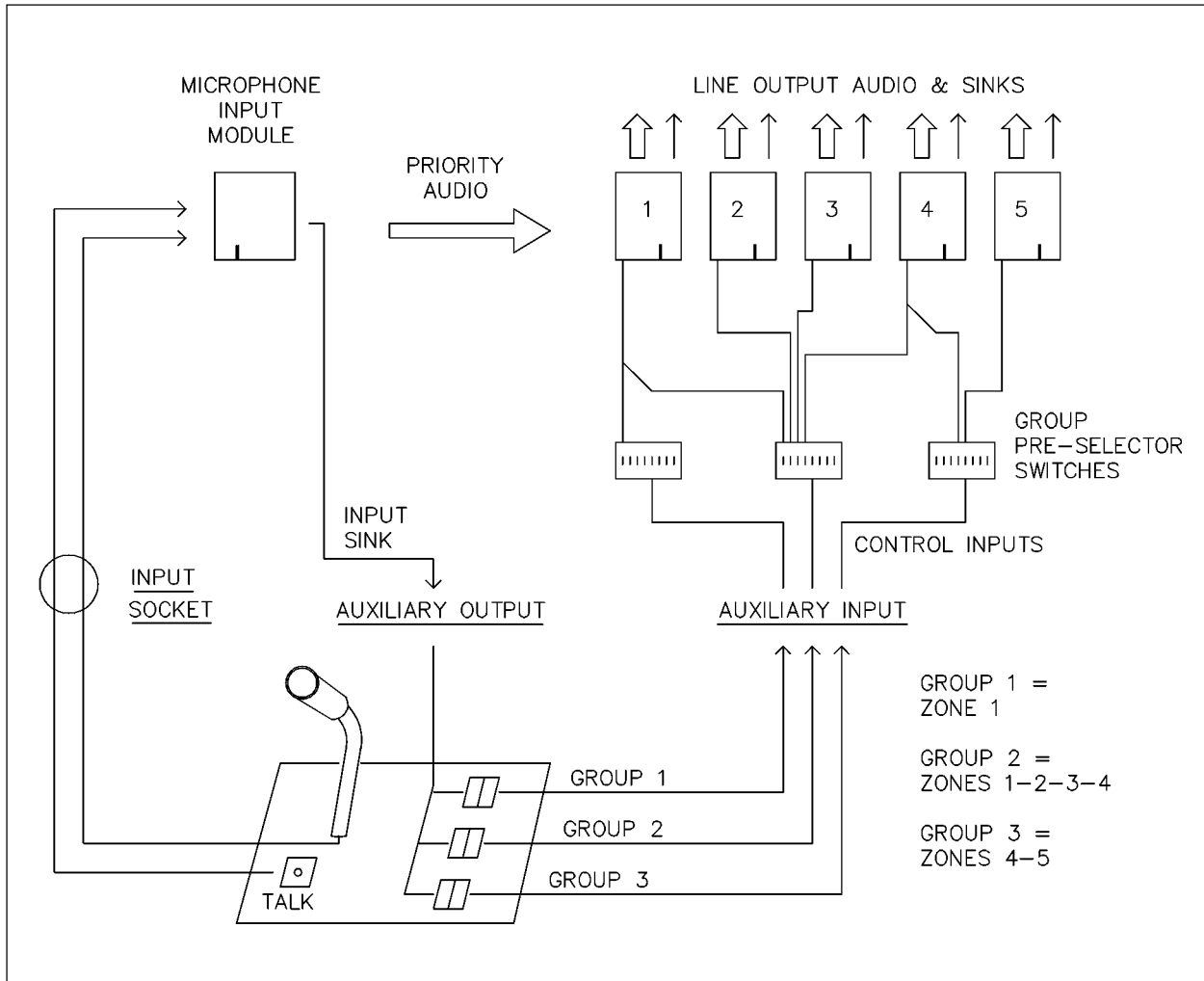
Fig. 8 General control concepts for ZG units
