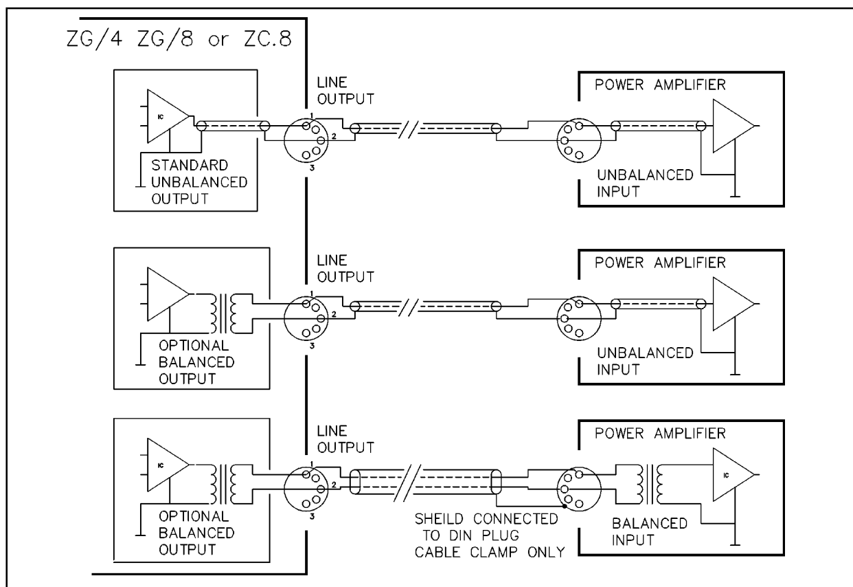
Fig. 11 Unbalanced and balanced line output connections
