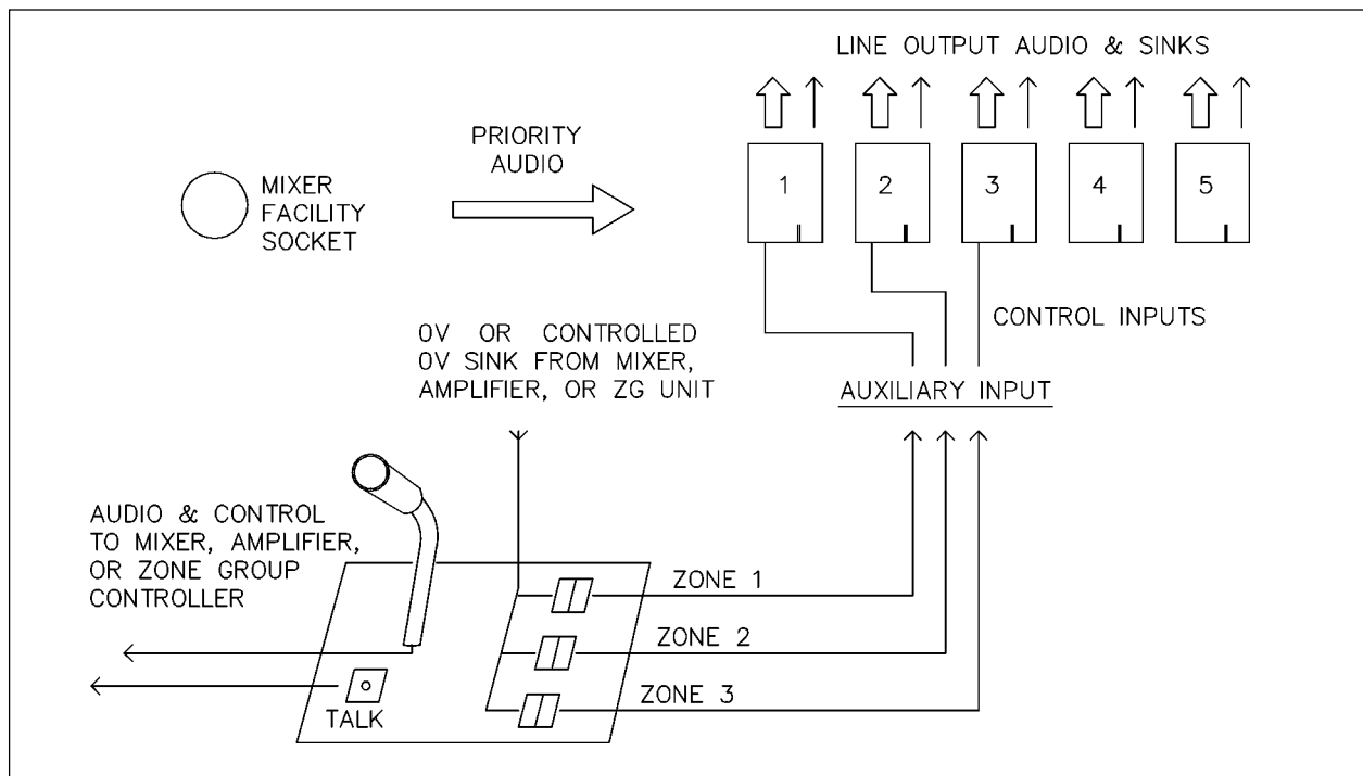
Fig. 9 General control concepts for ZC.8 units
