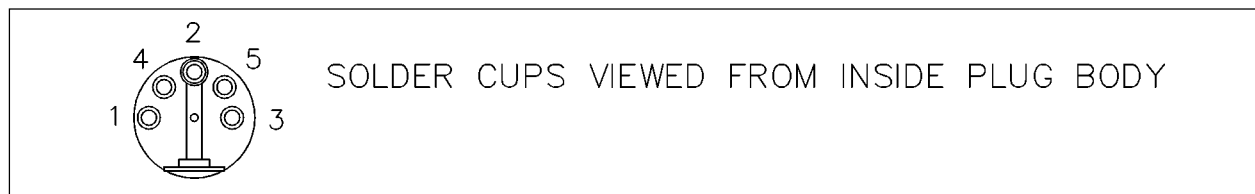
Fig. 2 DIN input connector pin identification - ZG units
